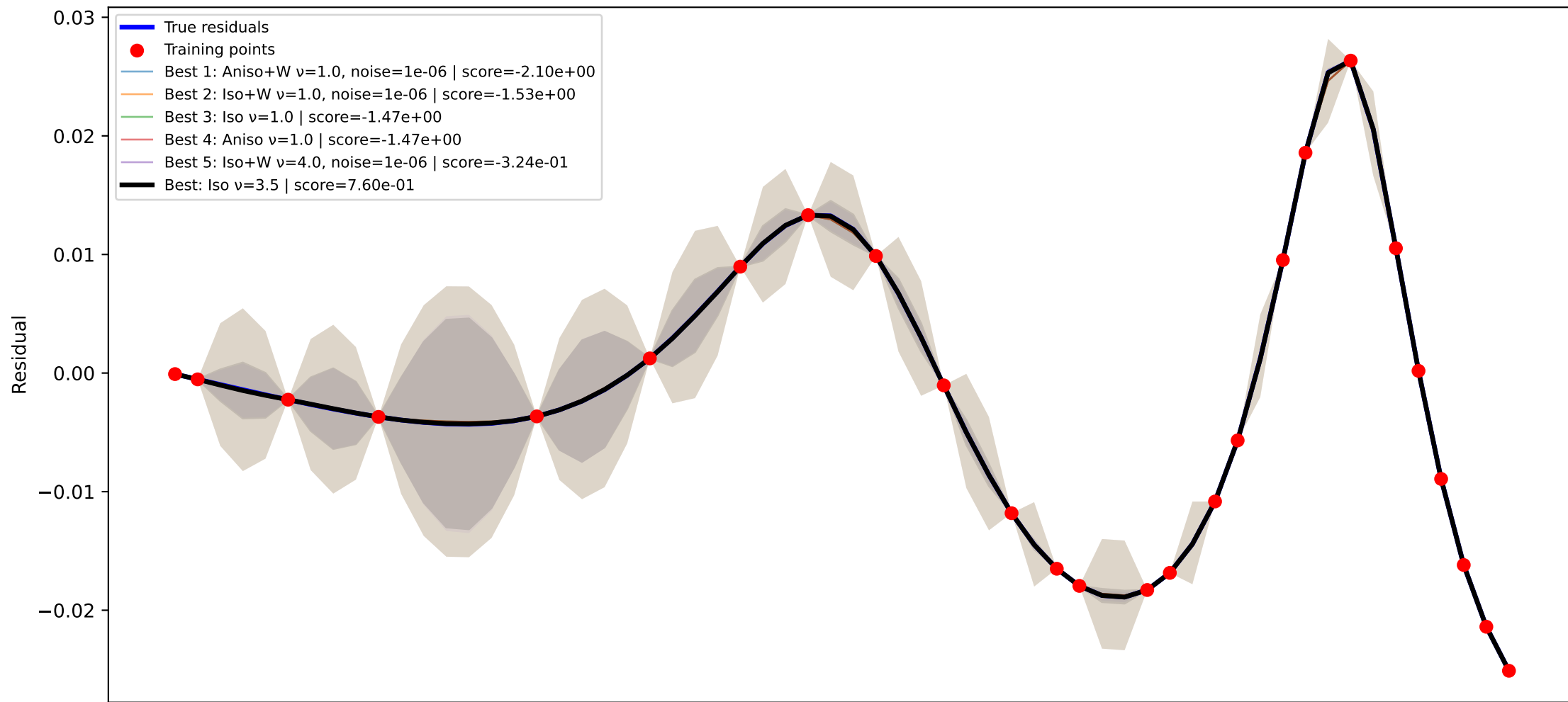
GPR kernel comparison node=11 RMSE=1.954e-05, train RMSE=2.341e-11
